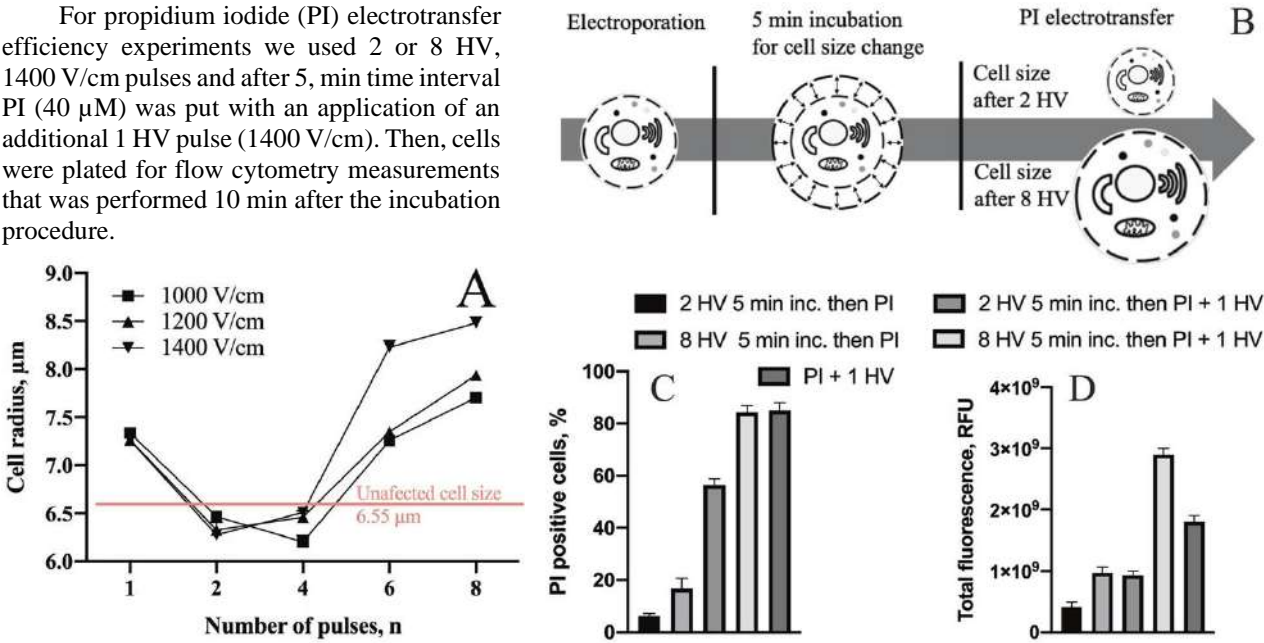
Fig. 1. A) Cell radii change after EP with 1-8 pulses at amplitude 1000 to 1400 V/cm for 100 µs. B) The scheme of used experiment setup. C) and D) PI positive cells and total PI fluorescence after ET using scheme as shown in part B. HV is coded as 1400 V/cm 100 µs pulse.
