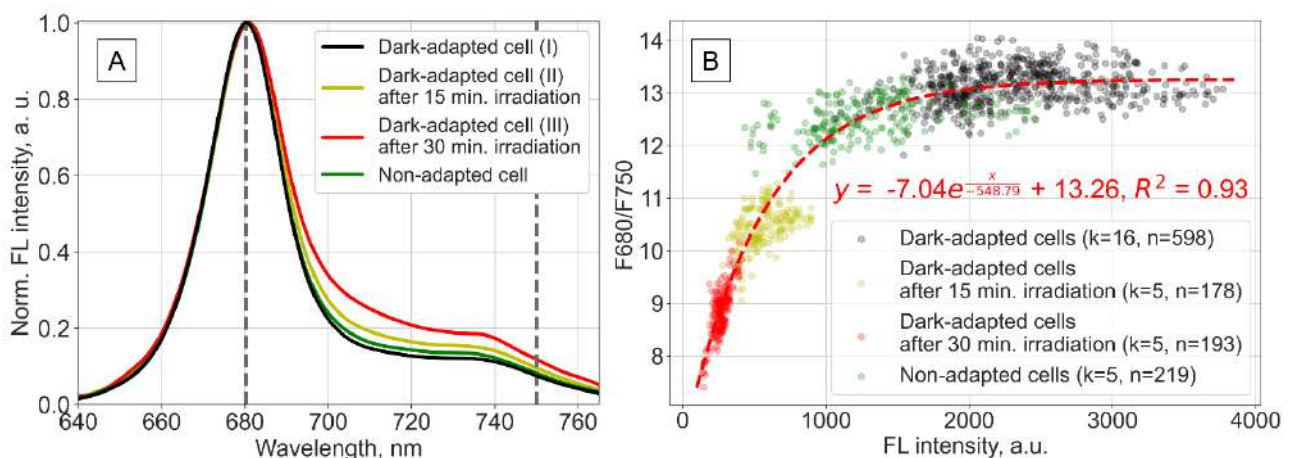
Fig. 1. Fluorescence (FL) spectra (A) and the relationship between peak FL intensity (680 nm) and F680/F750 ratio (B) in Nitellopsis obtusa internodes kept under different lighting conditions; k – number of cells, n – number of registered spectra
