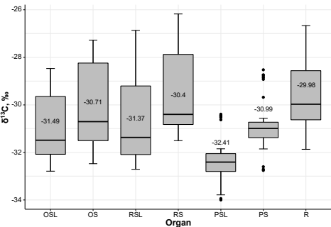
Fig. 1. \delta^{13}\text{C} in different Spinulum annotinum organs. Boxes represent the interquartile range (IQR) between the 1st (Q1) and the 3rd (Q3) quartiles. The line in the middle of the box shows the median, along with the median value. The lower whisker marks Q1–1.5IQR, the upper whisker – Q3+1.5IQR. Dots represent outliers.
